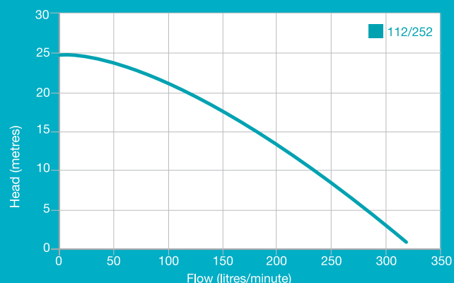
• Hi-Flo 112 / 252 Performance
